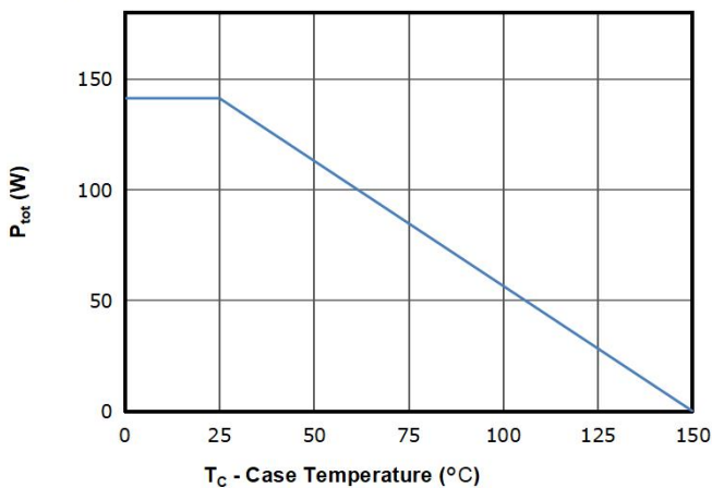
Fig 11: Power Dissipation
